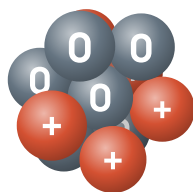
carbon-12
